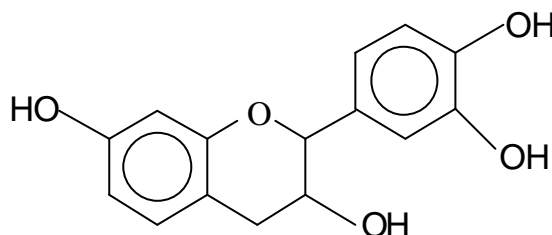
FLAVAN-3-OL
